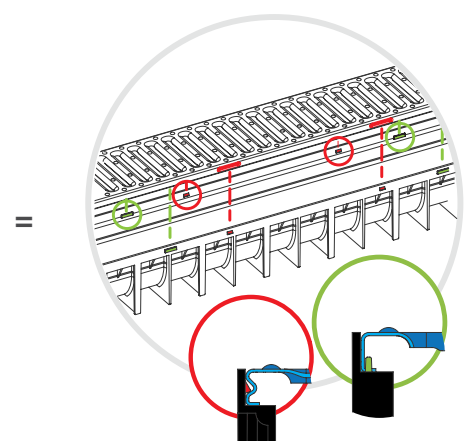
PROTRUSION DETAILS
